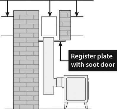
Horizontal register plate with rear flue connection
