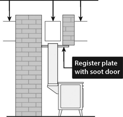
Horizontal register plate with optional vertical rear flue connection
