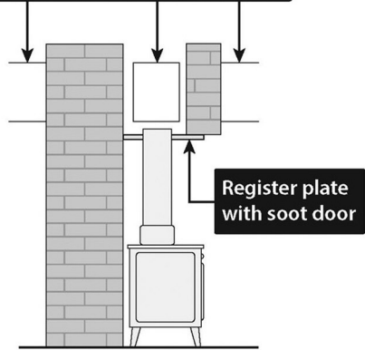
Horizontal register plate with top flue connection
