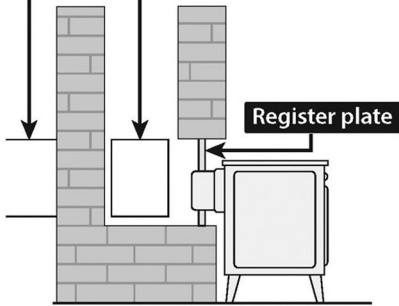
Vertical register plate with bricked-up fireplace
